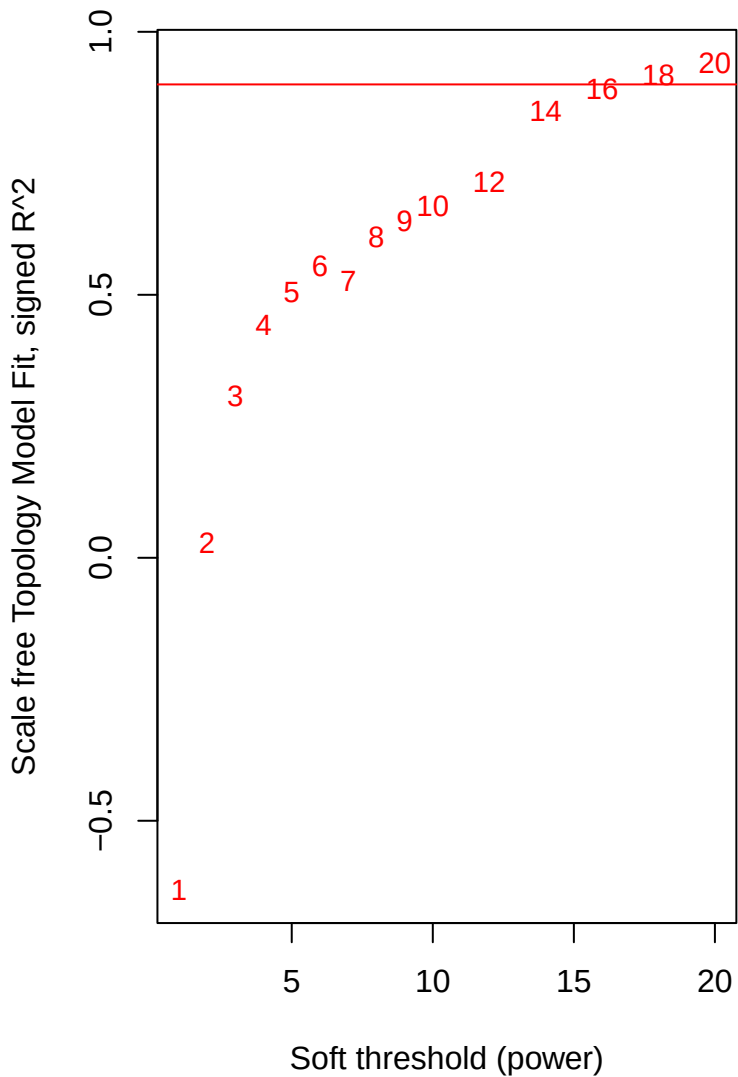
Scale independence
