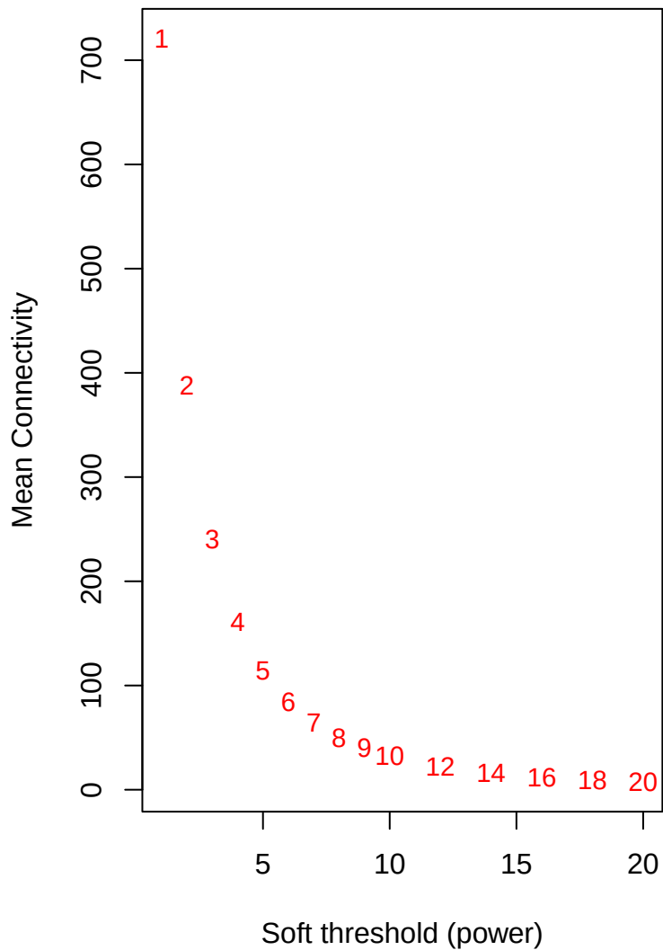
Mean connectivity
